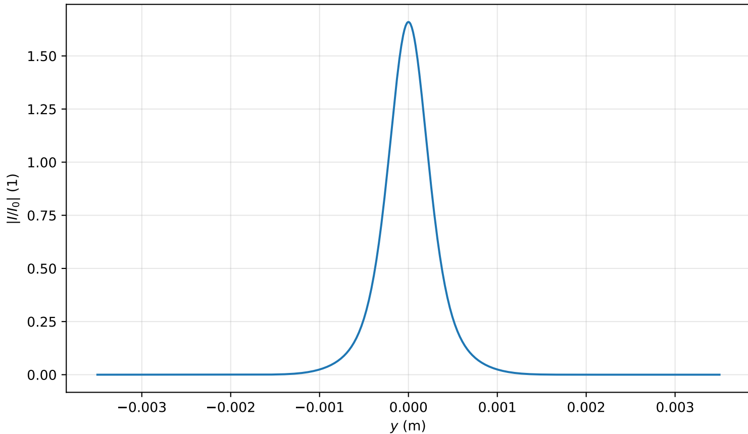
Intensity profile I(x=0, y, z=1.194)/I_0 , P_{in}=1.0P_{cr} , artificial time
